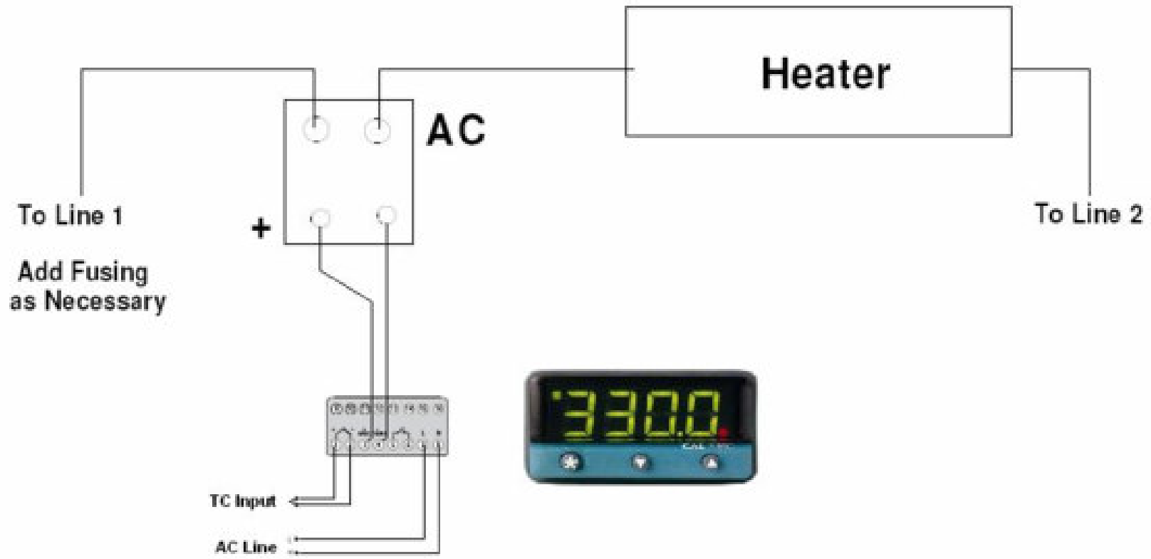
CAL 3300 Temperature Controller
